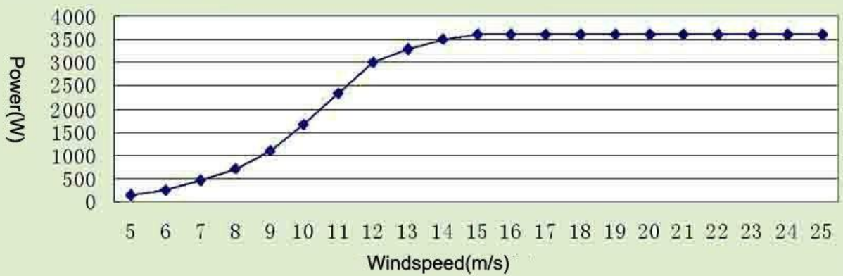
CWE-3 KW VAWT
