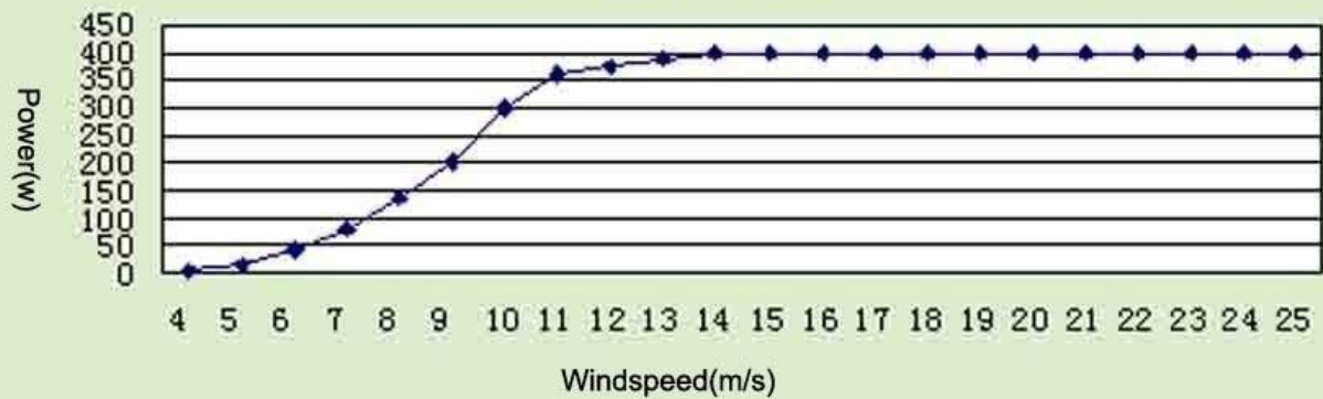
Windspeed/Power Curve
