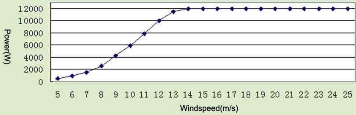
Windspeed/Power Curve
